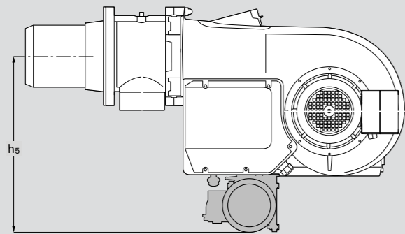
Motorised oil pump (Standard on WM 30/3)
