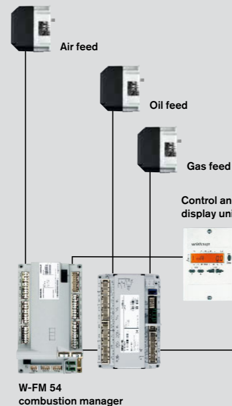
Schematic representation with W-FM 54
