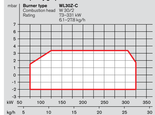
WL30 capacity graph
