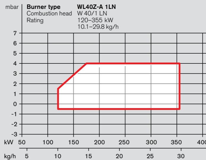
WL40 capacity graph
