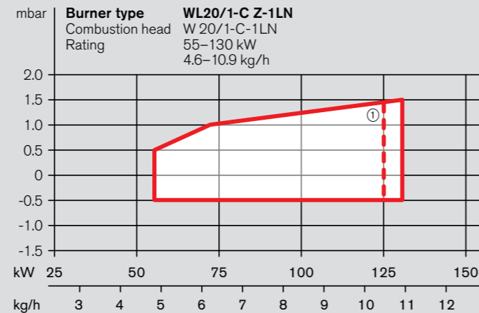
WL20 capacity graph
