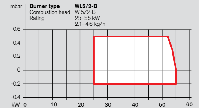
WL5 capacity graph
