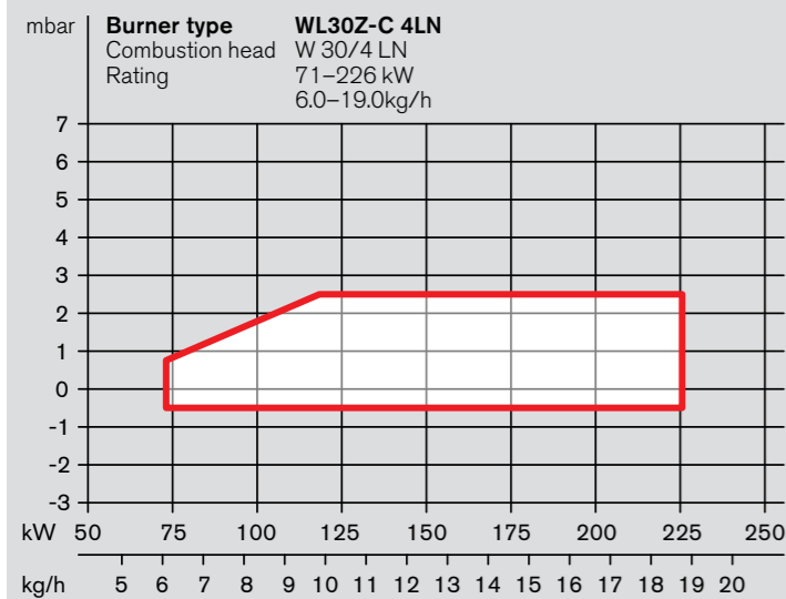
WL30 capacity graph
