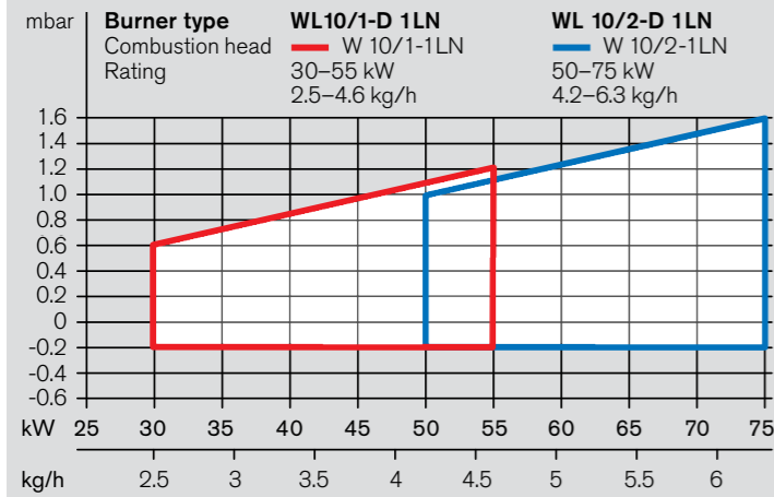
WL10 capacity graph
