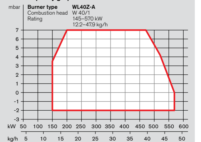
WL40 capacity graph
